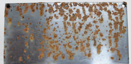
After 192 hours in a humidity cabinet, the metal coupon treated with a leading competitive product rusted severely.
